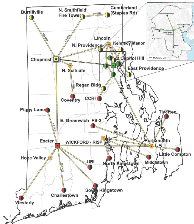
Figure 13.1.1-3: RISCON Network Deployment Map
