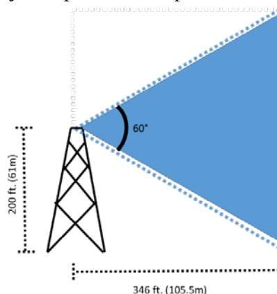
Figure 2.4.3-2: Depection of Primary Radiation Lobe of a Panel Antenna Attached to a 200 ft (61 m) Cell Tower
