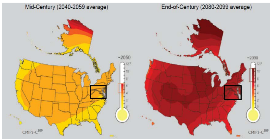
Figure 5.2.14-2: District of Columbia High Emission Scenario Projected Temperature Change
