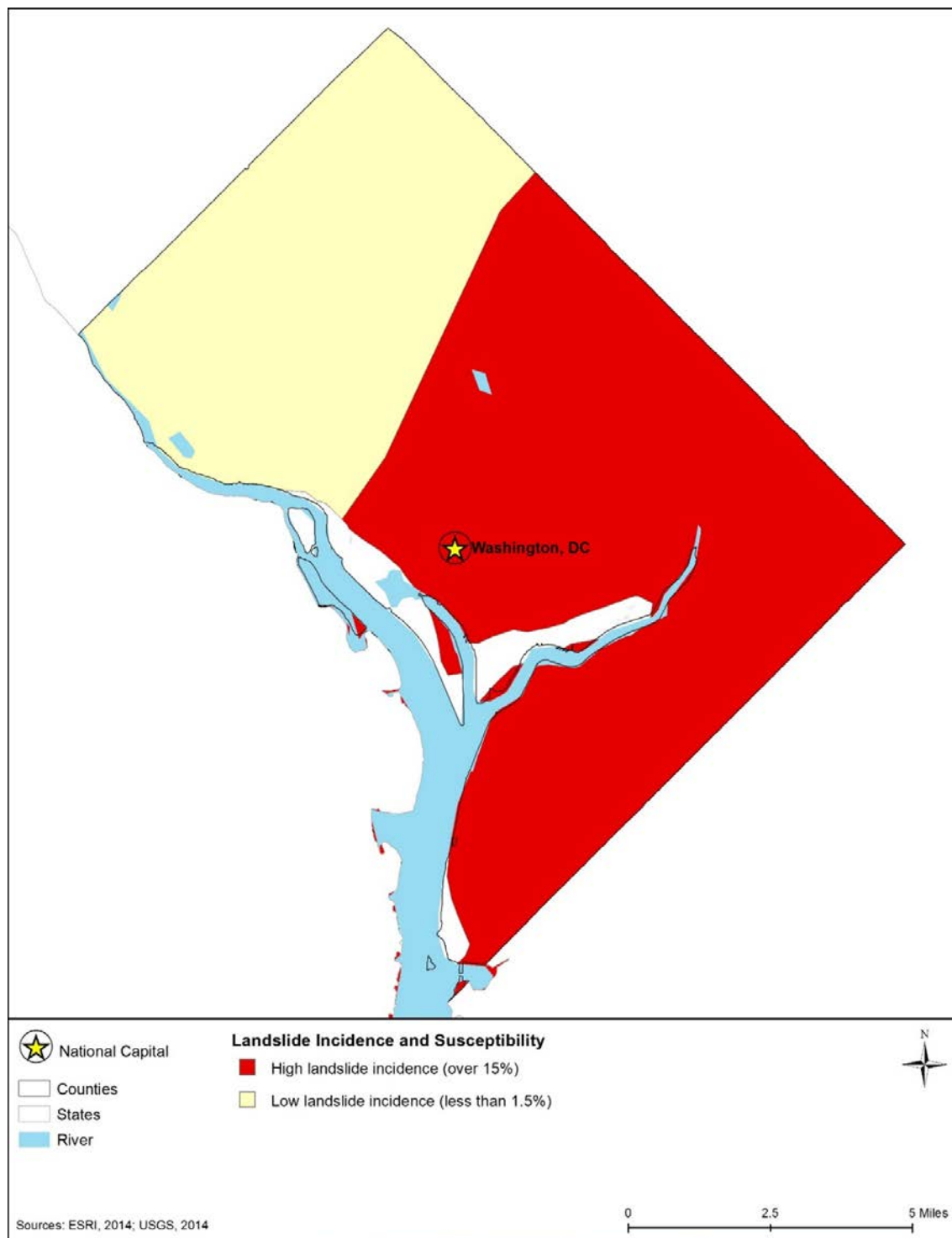
Figure 5.1.3-5: District of Columbia Landslide Incidence and Susceptibility Hazard Map 56
