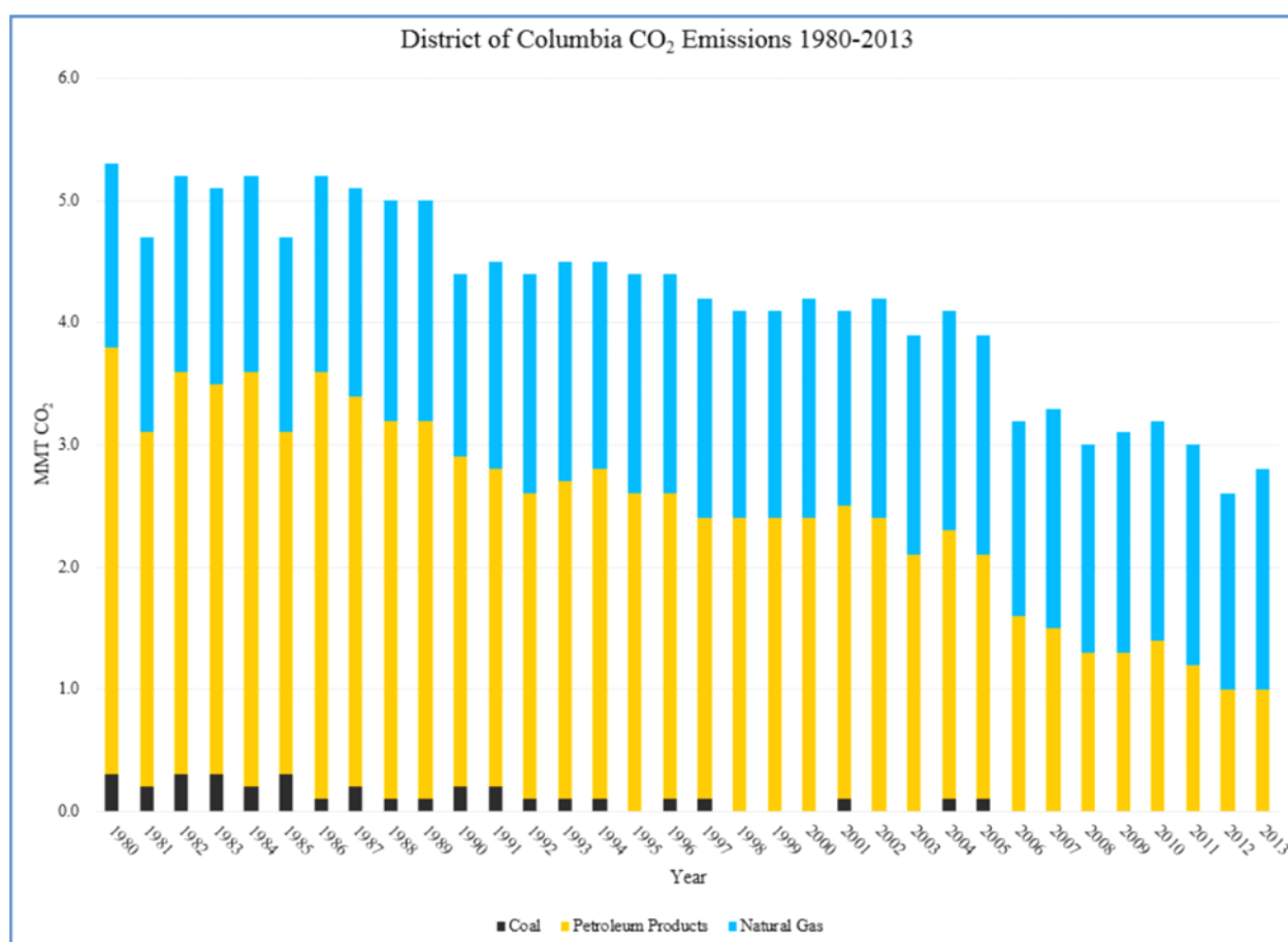
Figure 5.1.14-1: District of Columbia CO 2 Emissions from Fossil Fuels by Fuel Type 1980-2013
