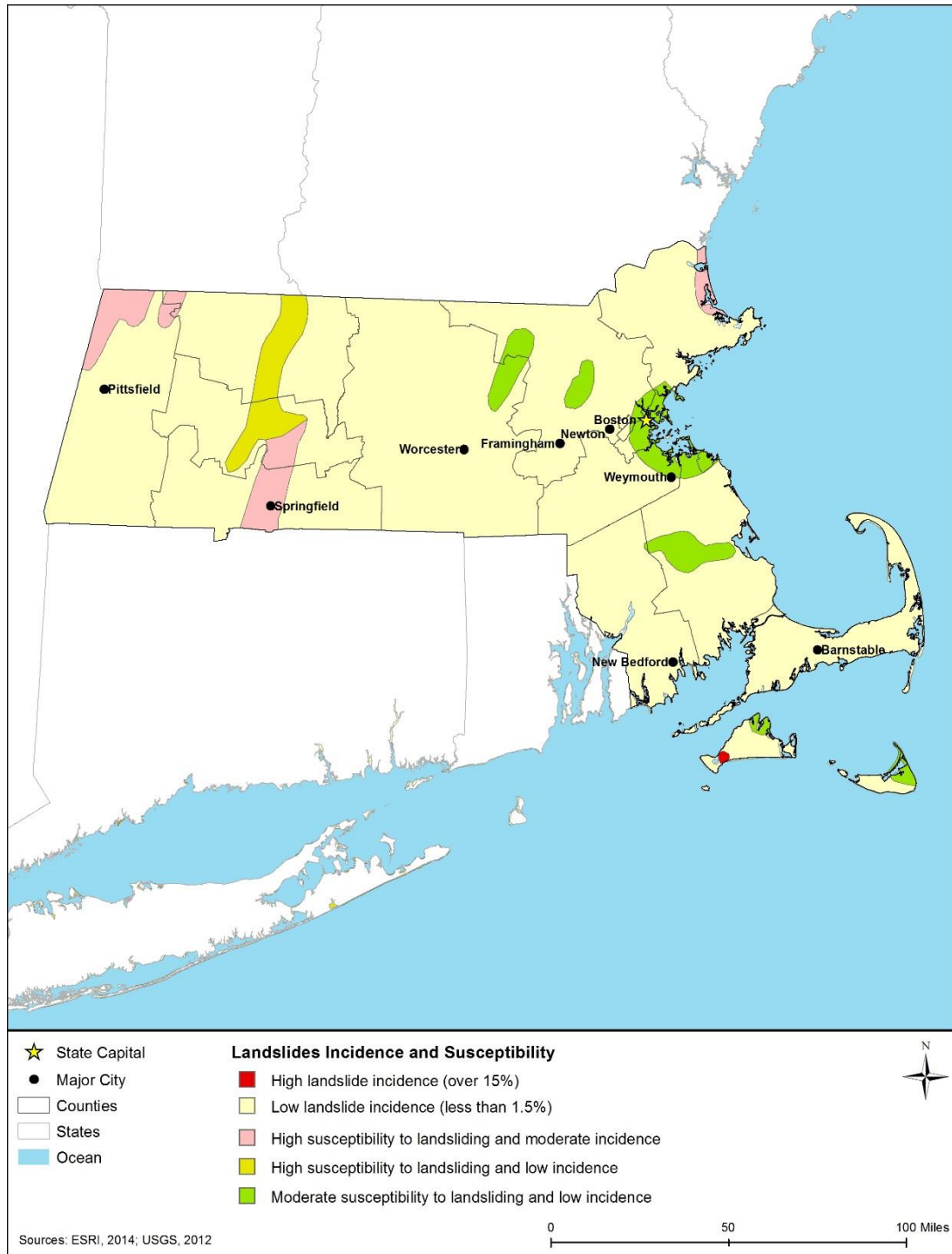
Figure 8.1.3-6: Massachusetts Landslide Incidence and Susceptibility Hazard Map 48
