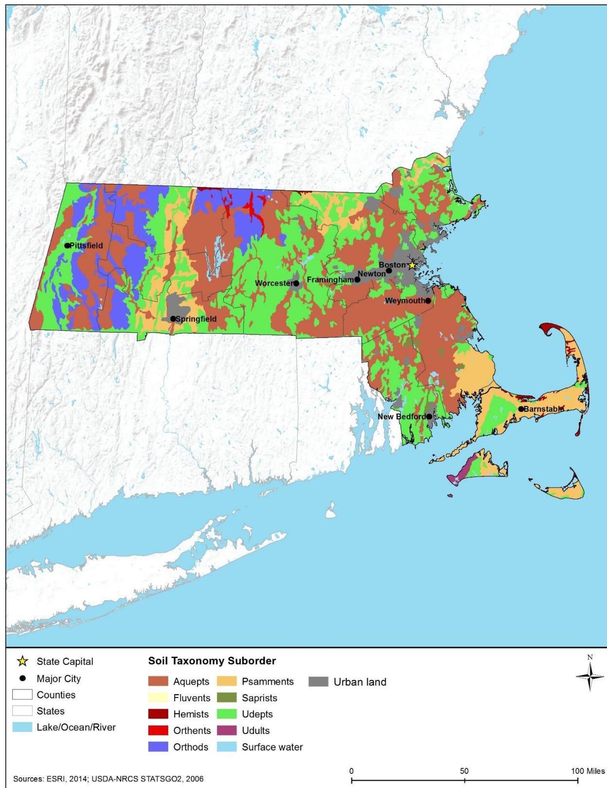
Figure 8.1.2-2: Massachusetts Soil Taxonomy Suborders
