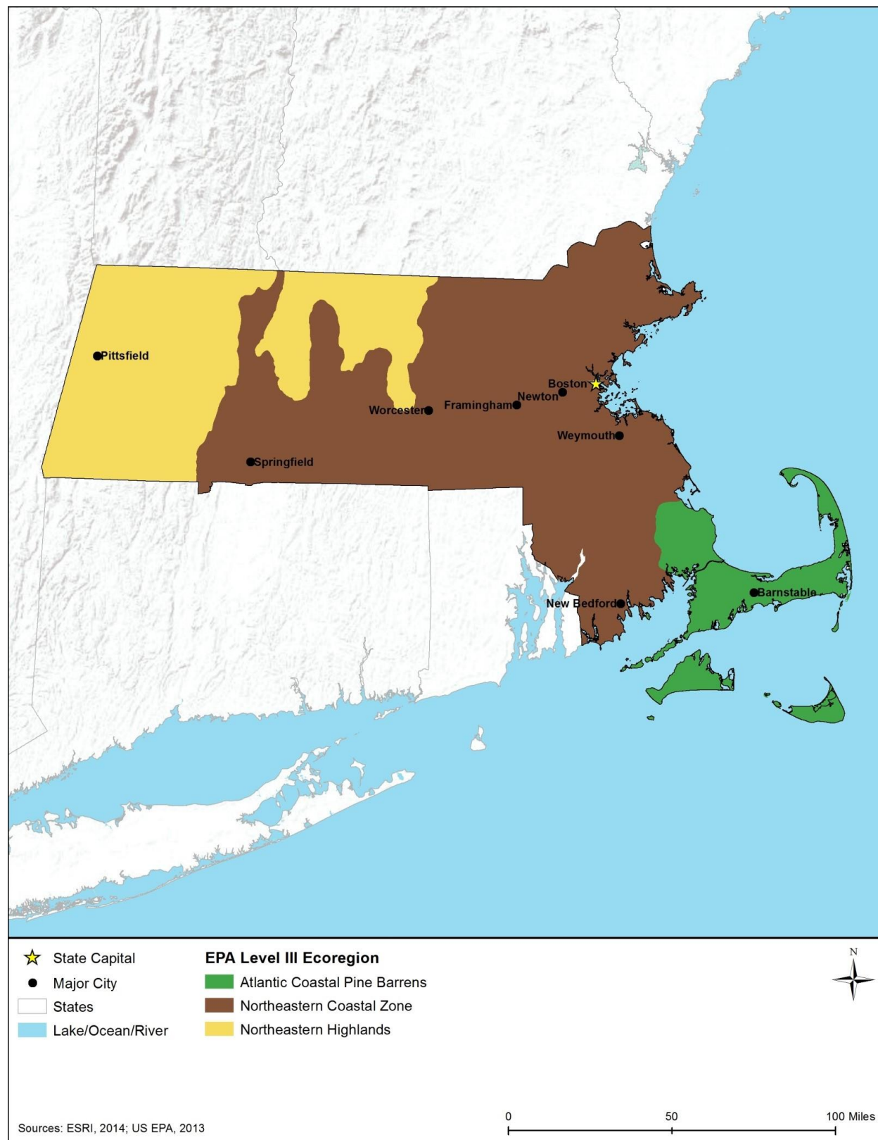
Figure 8.1.6-1: USEPA Level III Ecoregions in Massachusetts
