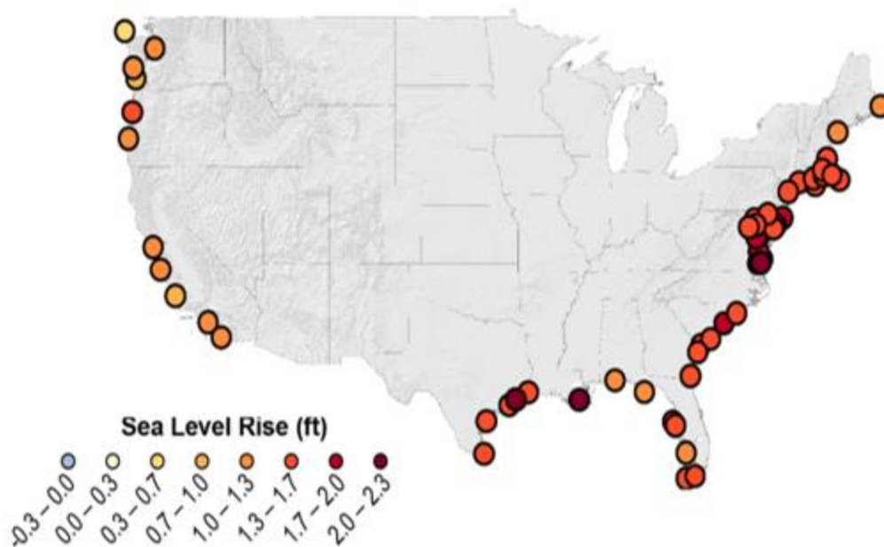
Figure 8.2.14-6: 1.24-foot Sea Level Rise Above 1992 Levels by 2050
