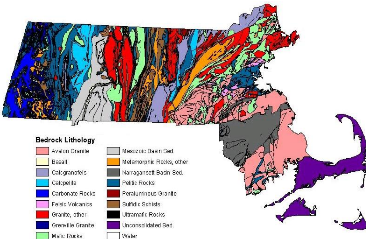
Figure 8.1.3-3: Generalized Bedrock Geology for Massachusetts
