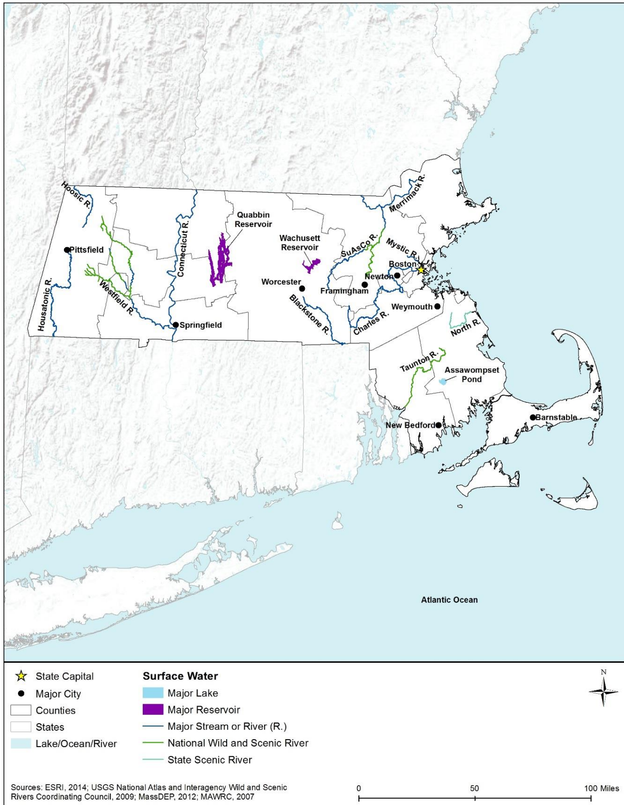
Figure 8.1.4-2: Major Massachusetts Surface Waterbodies
