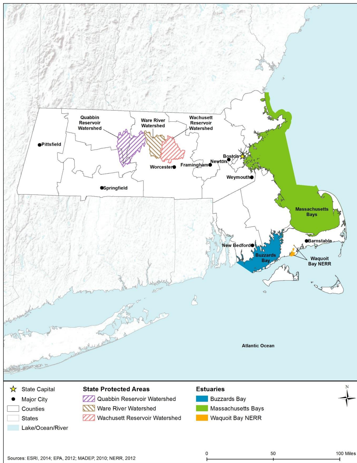
Figure 8.1.4-3: Massachusetts's Estuaries and Protected Waterbodies
