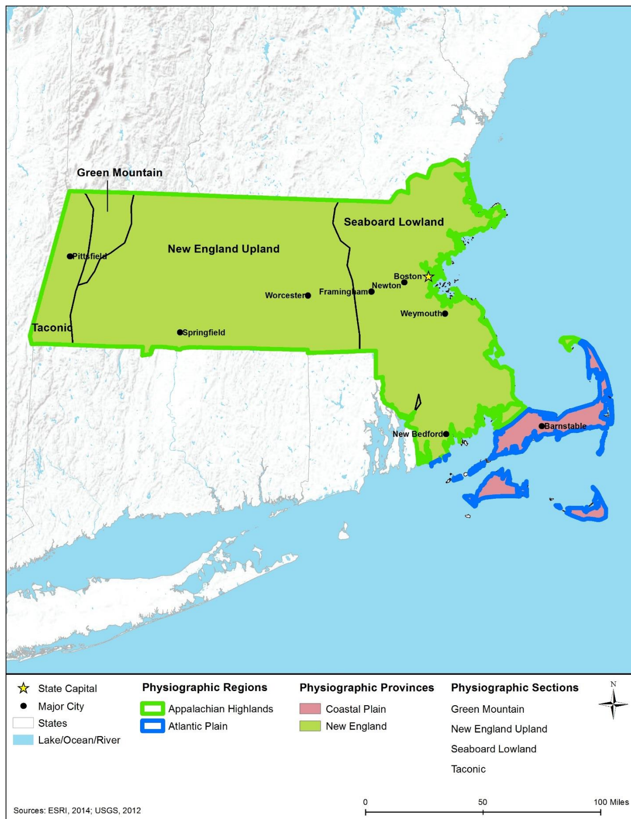
Figure 8.1.3-1: Physiographic Regions, Provinces, and Sections of Massachusetts
