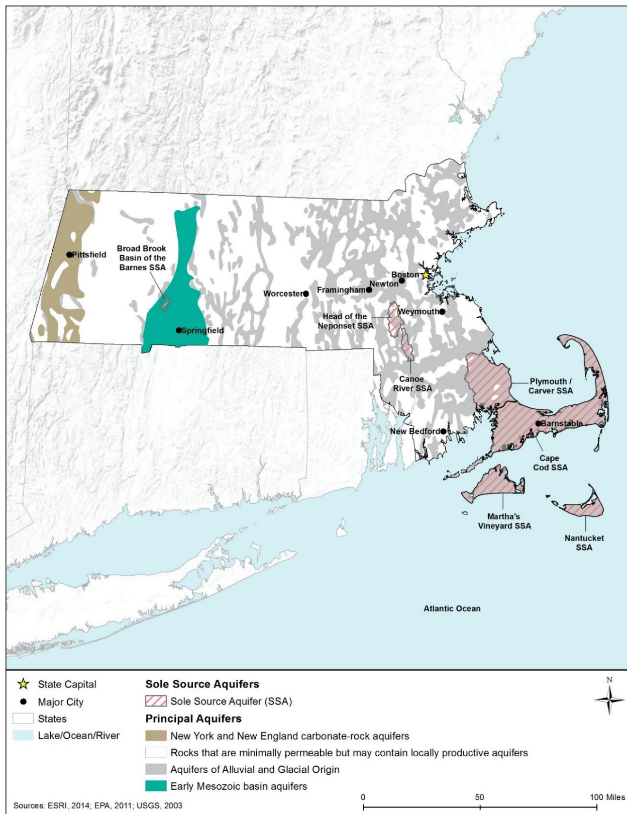
Figure 8.1.4-7: Principal and Sole Source Aquifers of Massachusetts
