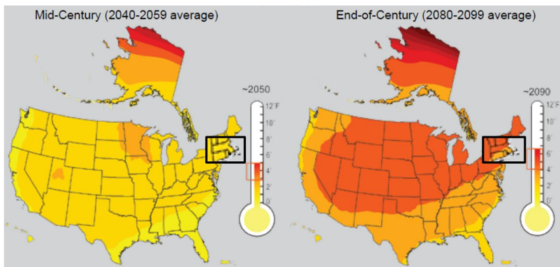
Figure 8.2.14-1: Massachusetts Low Emission Scenario Projected Temperature Change
