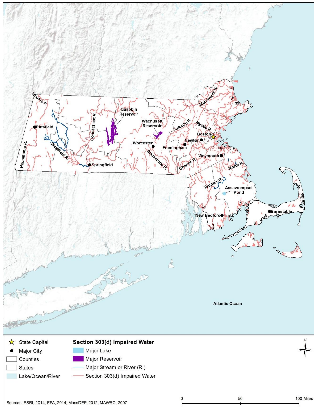
Figure 8.1.4-5: Section 303(d) Impaired Waters of Massachusetts, 2012
