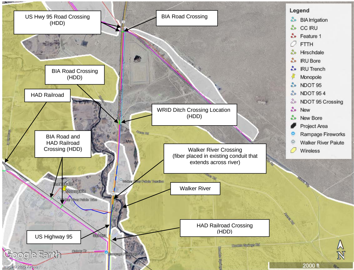
Figure 3-5 FTTH Road, Railroad, River, and WRID Ditch Crossing Locations
